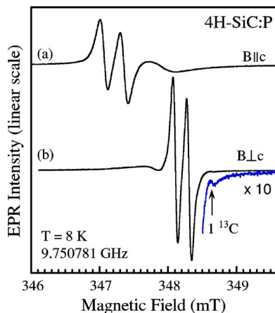
FIG. 15. (Color online) EPR spectra in P-doped 4H-SiC free-standing layers measured at 8 K for (a) \mathbf{B}\parallel\mathbf{c} and (b) \mathbf{B}\perp\mathbf{c} . The isotropic broad signal at \sim 347.85 mT is not related to the P_k center. The ^{13}\text{C} hf line of one nearest-neighbor C atom could be detected for the high-field line of the ^{31}\text{P} doublet.
