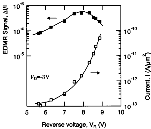
FIG. 3. Reverse-bias dependence of the EDMR signal and device current in a sample ( W=0.8 \mu\text{m} ). The signal intensity ( \Delta I/I ) is calculated from the higher-field-side peak height of signal B. Solid lines are guides to the eyes.
